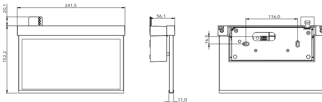
Dimensions GAMW wall mounting
