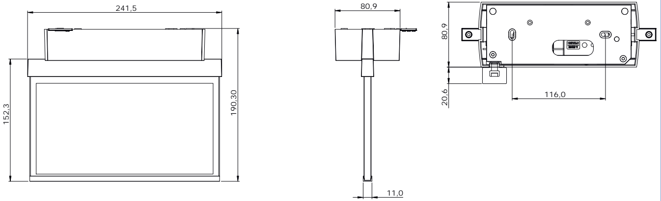
Dimensions GAMD ceiling mounting
