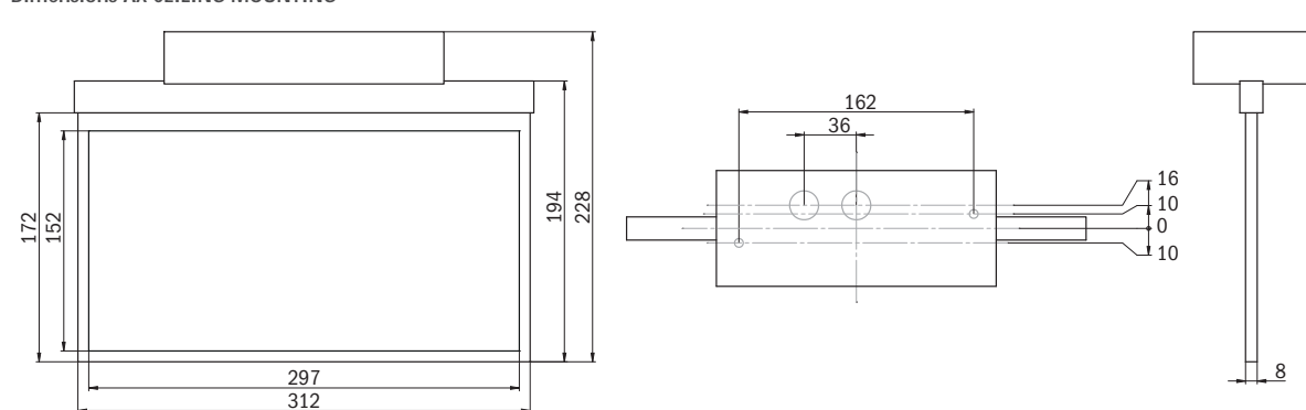
Dimensions AX CEILING MOUNTING
