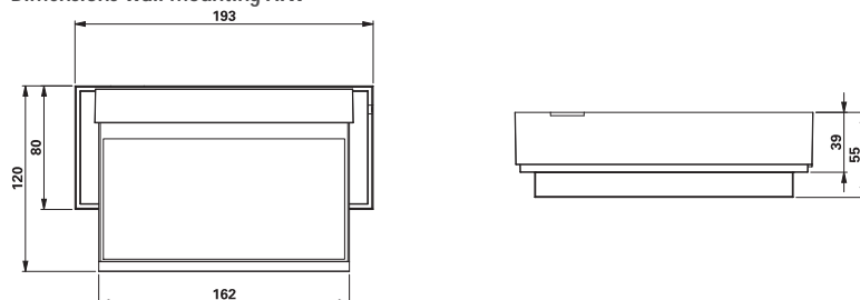
Dimensions wall mounting AIW
