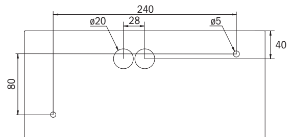
Drilling distances ZAW
