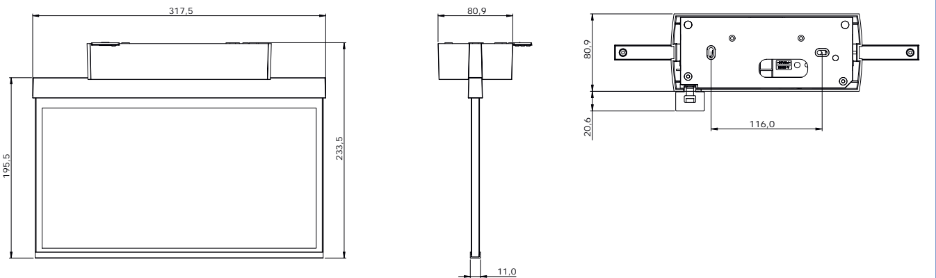
Dimensions GAXD ceiling mounting
