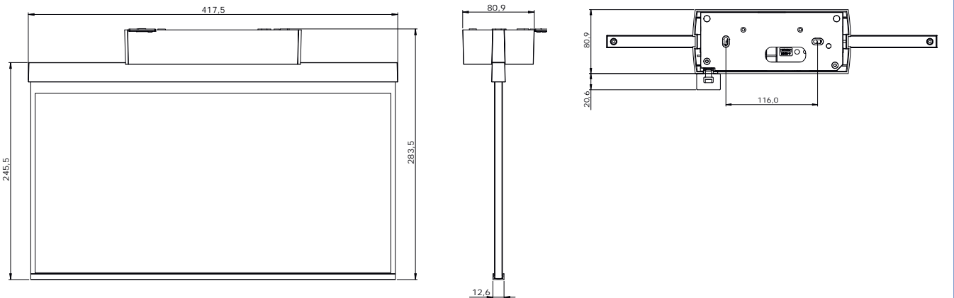
Dimensions GABD ceiling mounting
