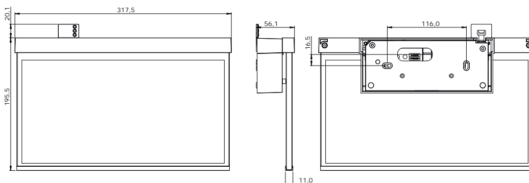
Dimensions GAXW wall mounting
