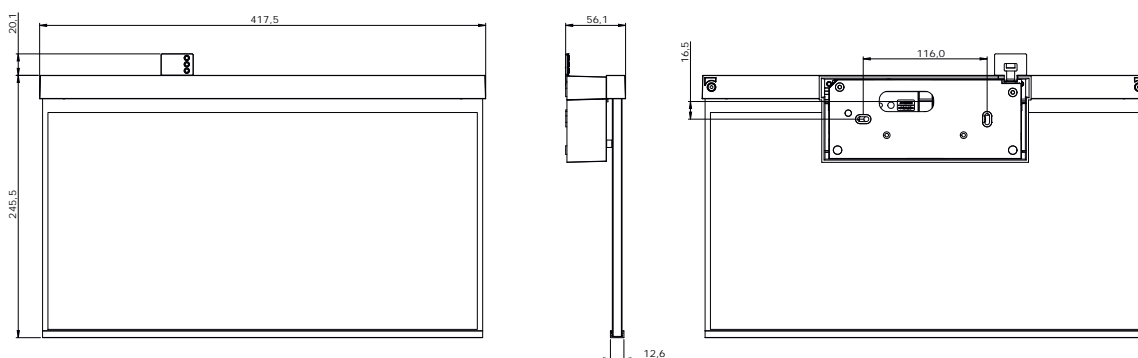
Dimensions GABW wall mounting
