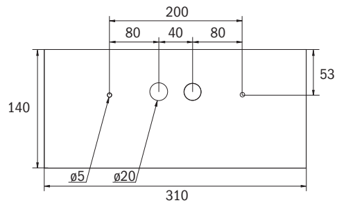
Drilling distances KC
