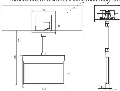
Dimensions AI recessed ceiling mounting AIEP
