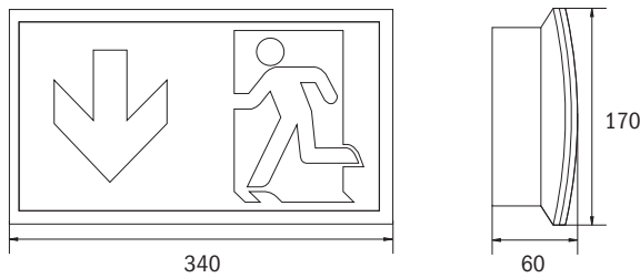
Dimensions KC wall
