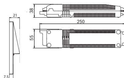
SelfContained electronics box (optional)
