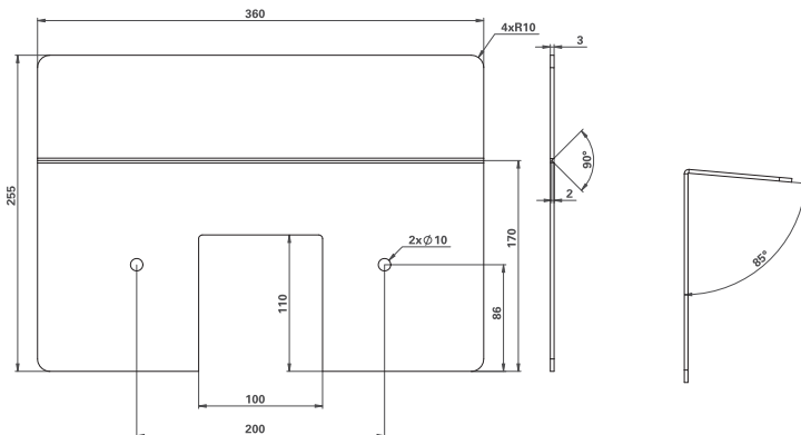
Rain cover KCRD for KCW (with IP65 Option only)
