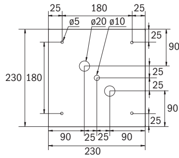
Drilling distances WG
