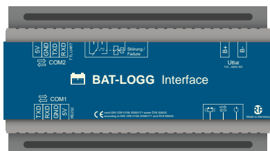
BAT-LOGG® Interface (DIN rail module: 156x86x58mm)
