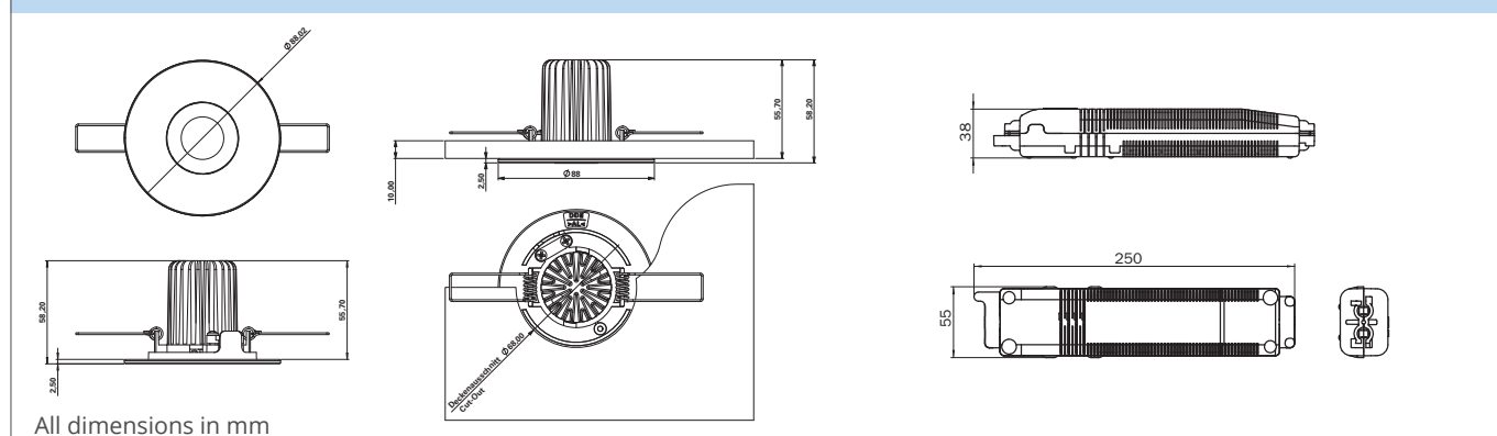
Distance Table for DDE039ML for plane emergency routes (additional distance tables on our website)
