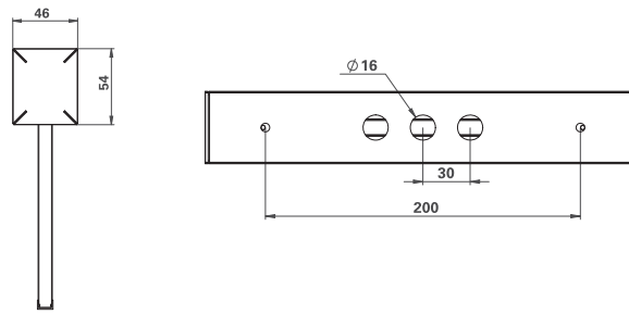
Drilling distances ASMU
