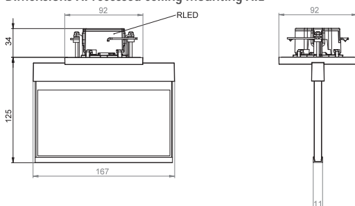
Dimensions AI recessed ceiling mounting AIE
