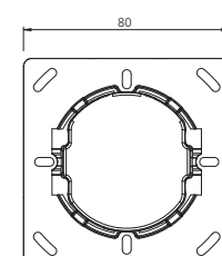
WER 029ML installation socket
